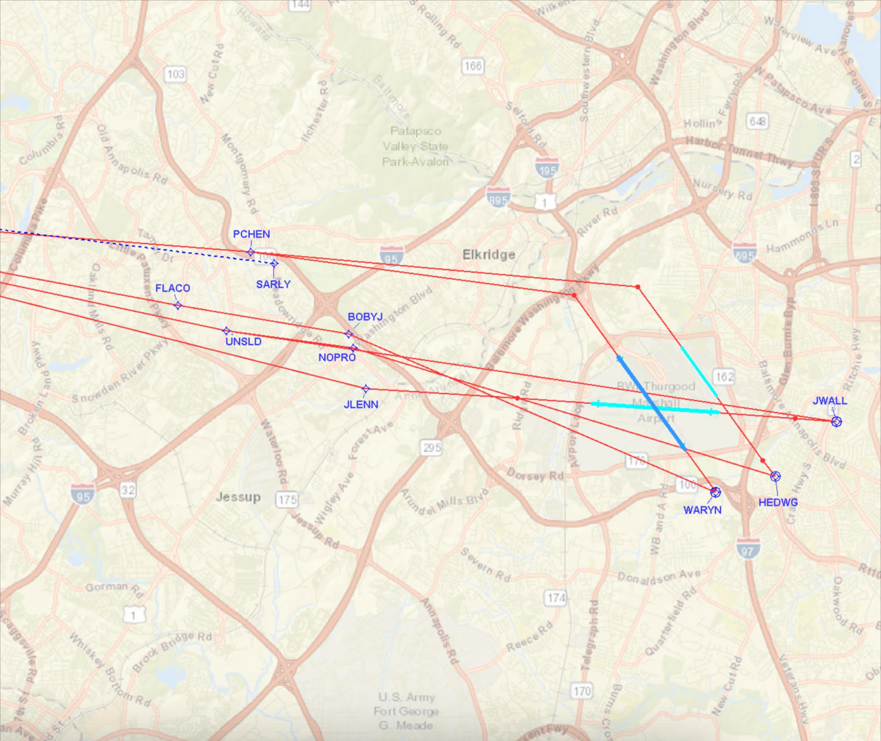
FOXHL Departure (Airport View)
