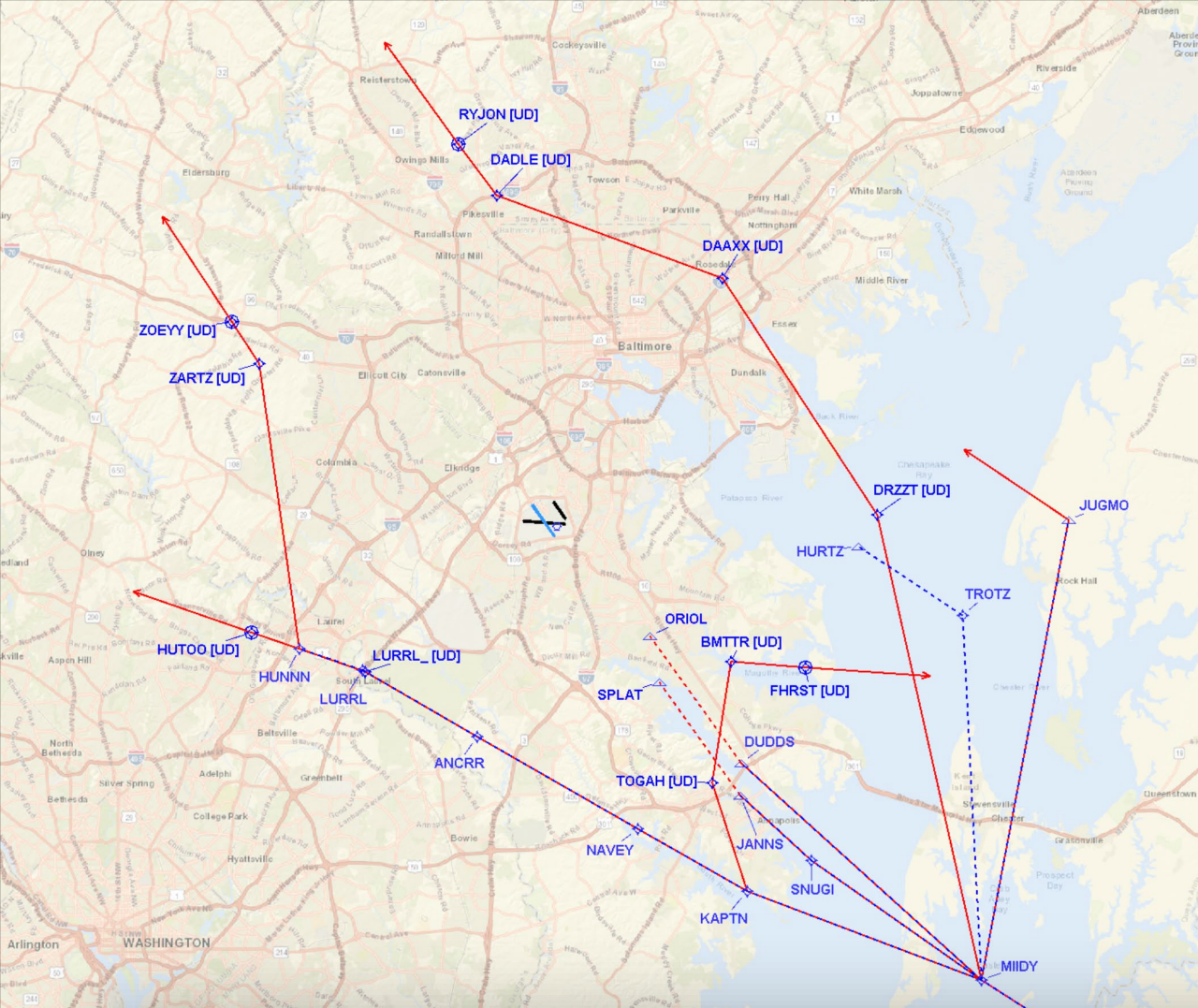
MIIDY Arrival (Runway Transitions)
