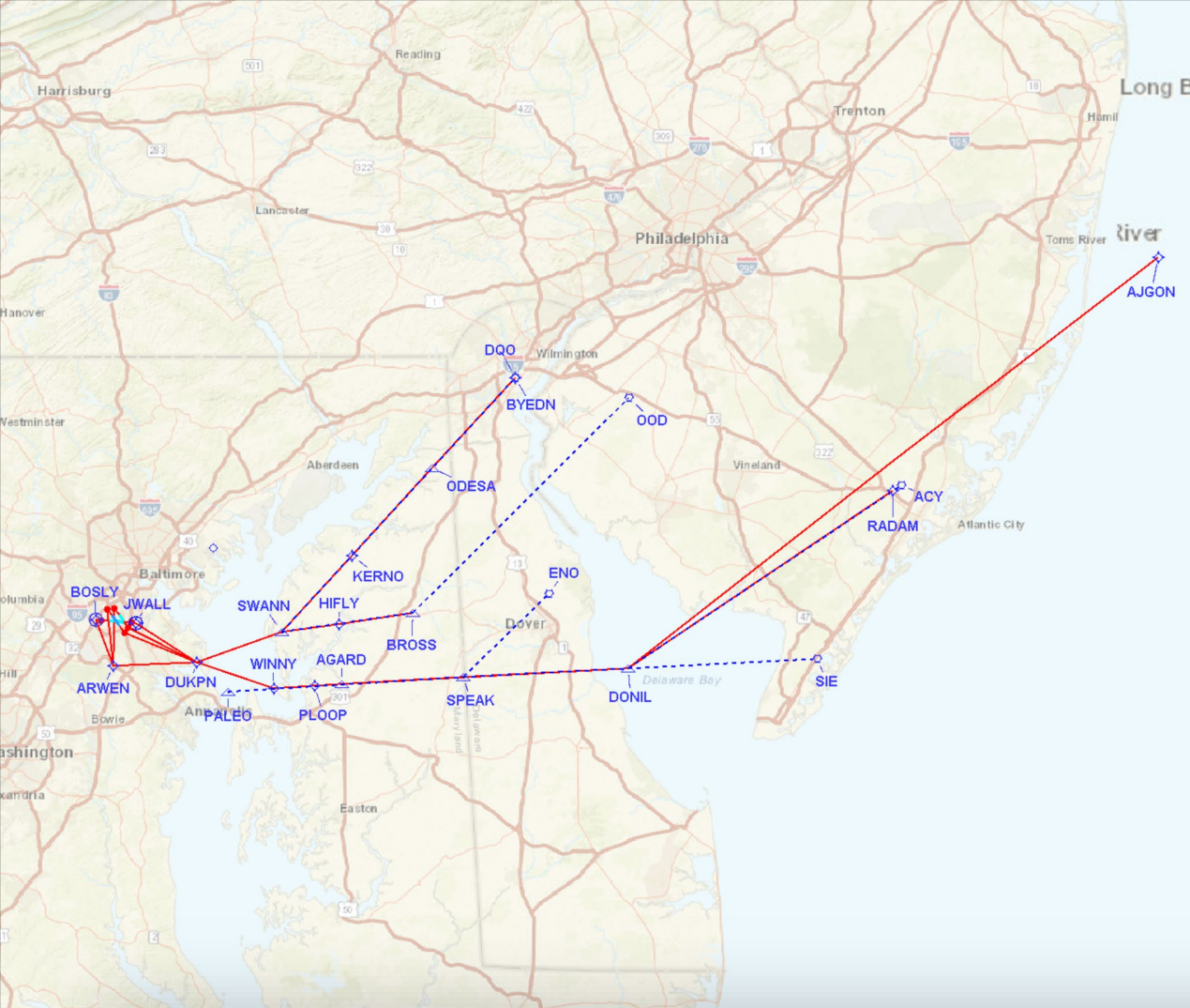
DUKPN Departure (Full Procedure)
