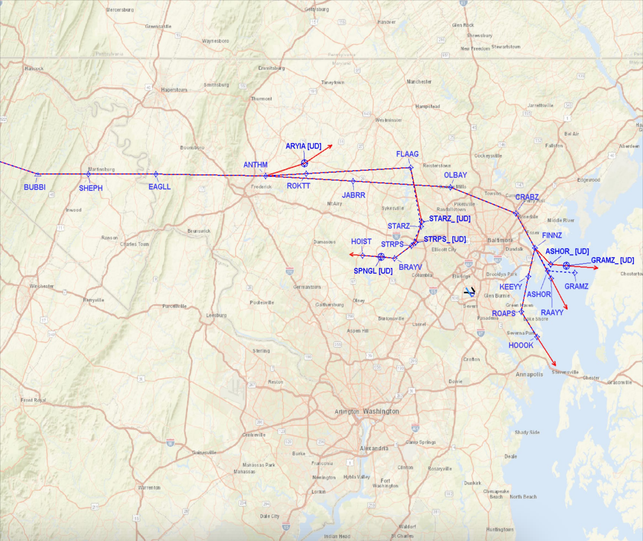
ANTHM Arrival (Common Route)
