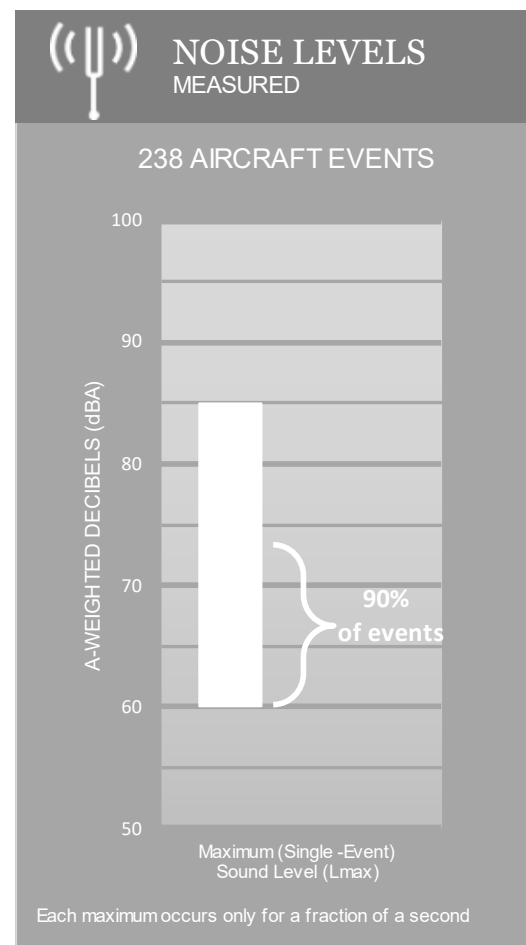
Figure 6. Maximum Single Event Aircraft Noise Levels
