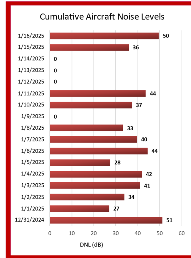
Figure 9. Measured Daily Aircraft Noise Levels
