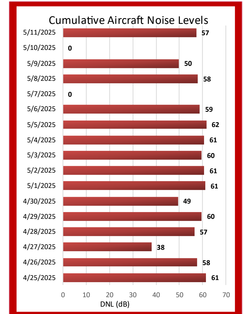
Figure 10. Measured Daily Aircraft Noise Levels April 25-May 11
