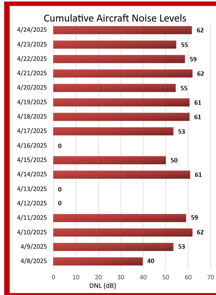
Figure 9. Measured Daily Aircraft Noise Levels April 8-April 24
